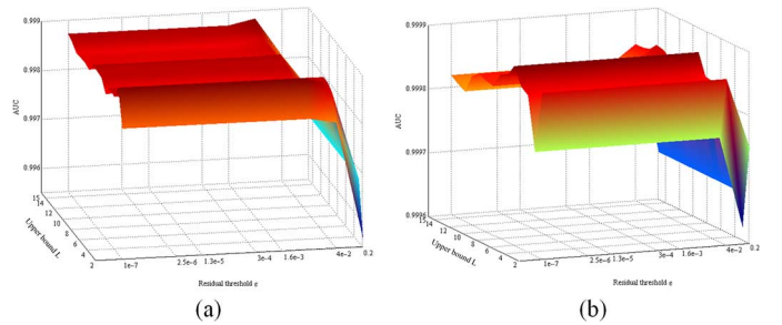
Fig. 11. AUC versus the SOMP-related parameters for the proposed algorithm with the two hyperspectral datasets. (a) HYDICE dataset. (b) Hyperion dataset.
