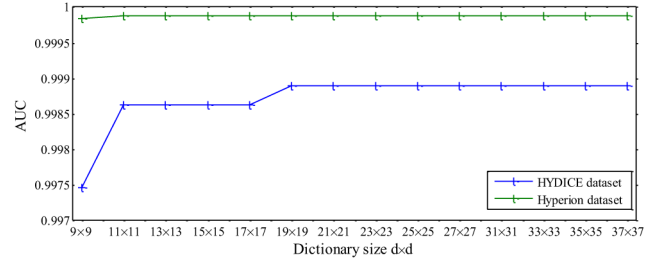
Fig. 10. AUC versus the local dictionary size for the proposed algorithm with the two hyperspectral datasets.
